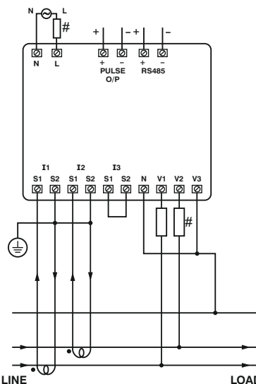
2 PHASE - 3 WIRE 2 Ø - 3 Wire, 2 CT'S
